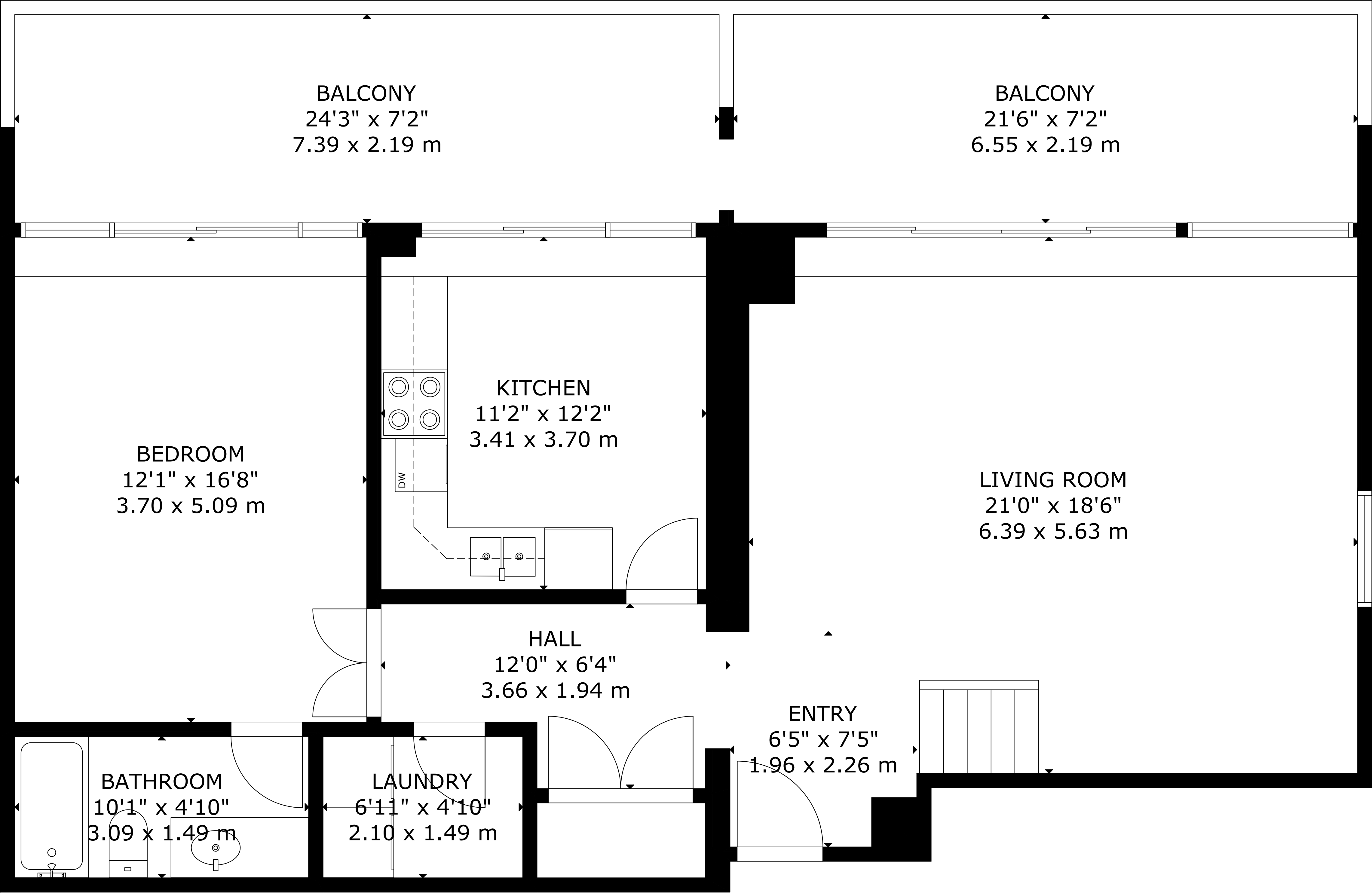
MAIN FLOOR
