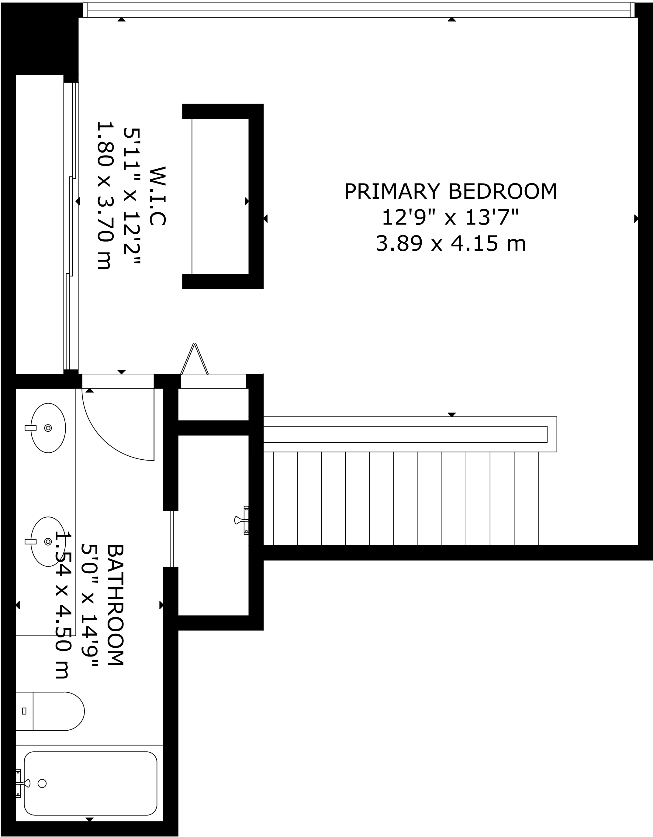
UPPER LEVEL 1
